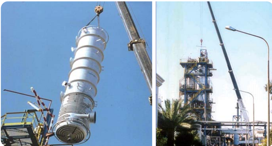
Project: Design and Fabrication of two columns, C101:Stripper gasoline C201:Oil regeneration Owner: SOTULUB (Tunisia) Year: 2001
